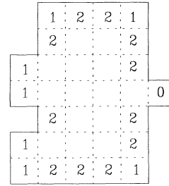
FIG. 2. To prevent topplings inside \mathcal{S} the boundary sites of \tilde{\mathcal{S}} cannot be larger than 3 minus the number of exterior neighbors. The figure displays a situation in which the boundary sites equal the maximum value. By inspection we see that the configuration \tilde{\mathcal{S}} is a forbidden subconfiguration, i.e., \tilde{\mathcal{S}} is not burnable.
