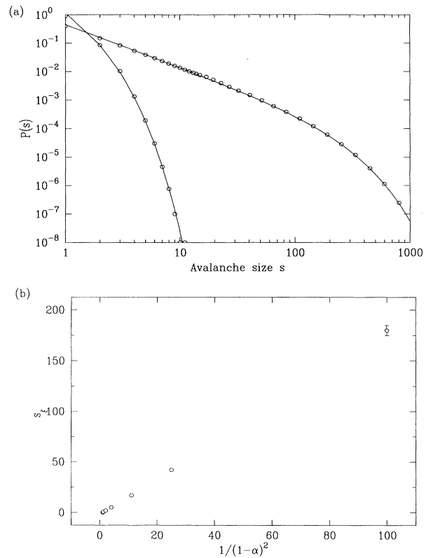
FIG. 1. (a) The measured distribution function of avalanche sizes in the annealed random-neighbor model with 2 and 18 neighbors. The solid lines show the analytical expression of Eq. (10) when we use s_\xi = 0.64 (2 neighbors) and 180 (18 neighbors). (b) The cutoff in cluster size distribution s_\xi as a function of 1/(1-\alpha)^2 .
